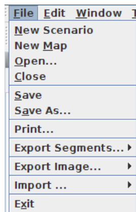
Figure 4.2: File Menu
