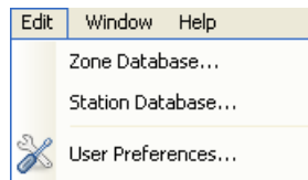
Figure 4.4: Edit Menu
