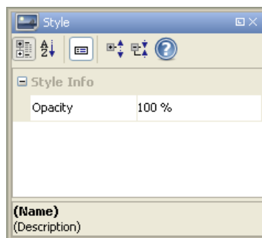
Figure 7.13: Style Toolwindow
