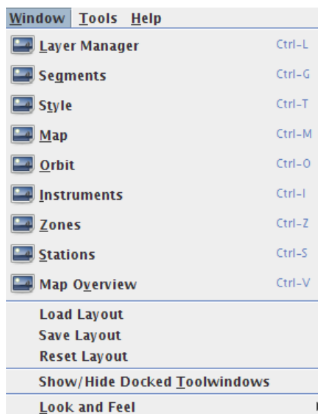
Figure 4.6: Window Menu
