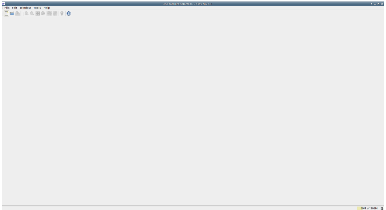
Figure 4.1: Main Window
