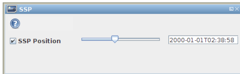
Figure 5.15: SSP Toolwindow
