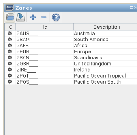
Figure 5.7: Zones Toolwindow
