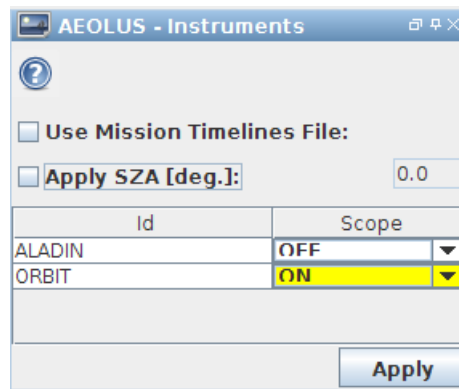
Figure 5.6: Instruments Toolwindow
