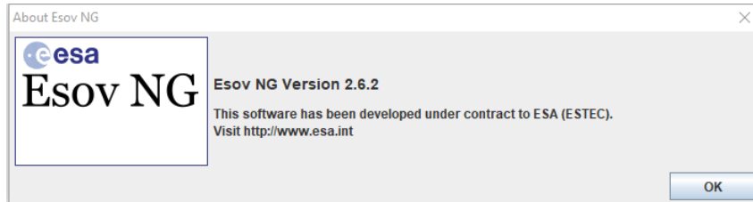
Figure 15.2: 'About' Dialog
