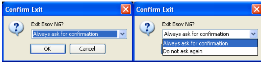
Figure 4.3: Exit Dialog
