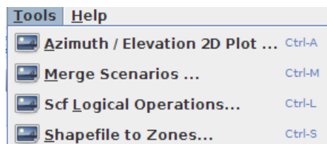
Figure 4.5: Tools Menu
