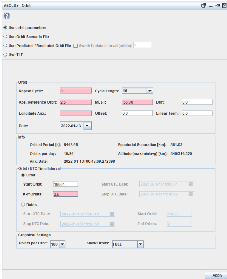
Figure 5.4: Invalid orbit definitions
