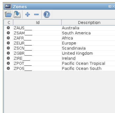
Figure 5.7: Zones Toolwindow
