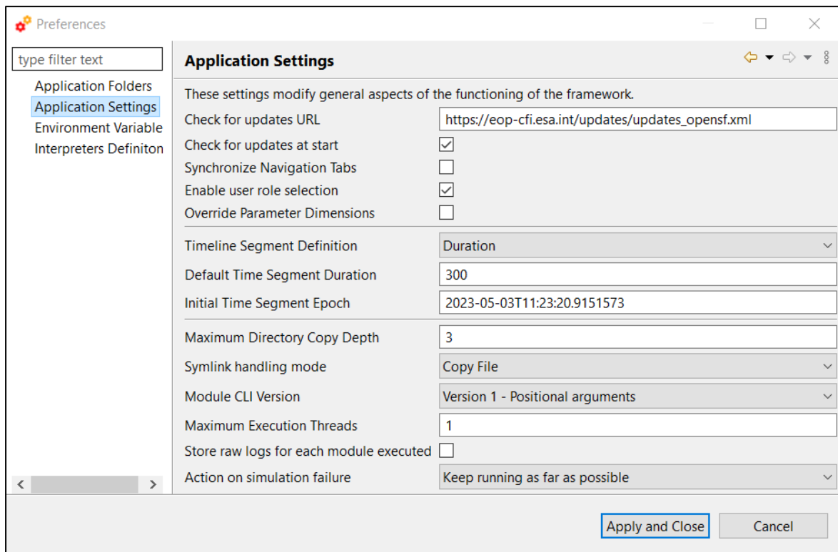
Figure 4-145: System Applications settings
