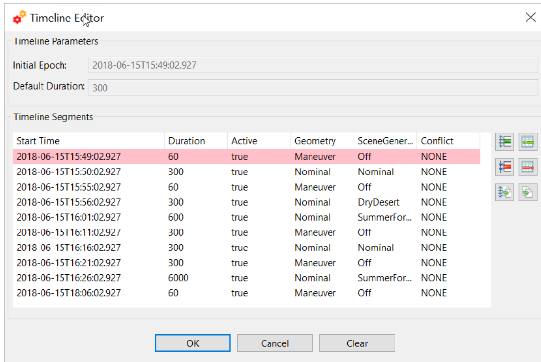
Figure 4-109: Timeline management view
