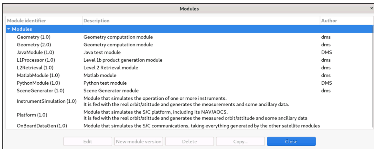
Figure 4-34: Module list view
