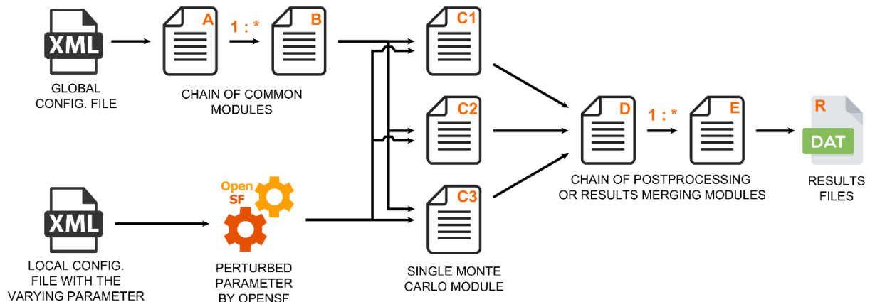
Figure 4-111: Monte Carlo chain in statistical mode
