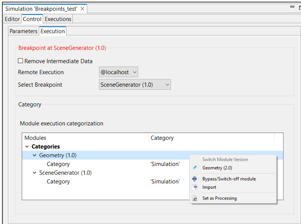
Figure 4-108: Module categorization by Mode
