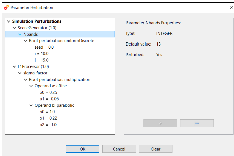
Figure 4-97: specific view of perturbations at parameter level
