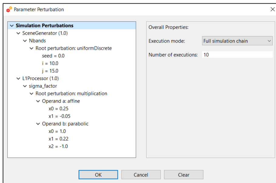
Figure 4-95: Perturbation system main window
