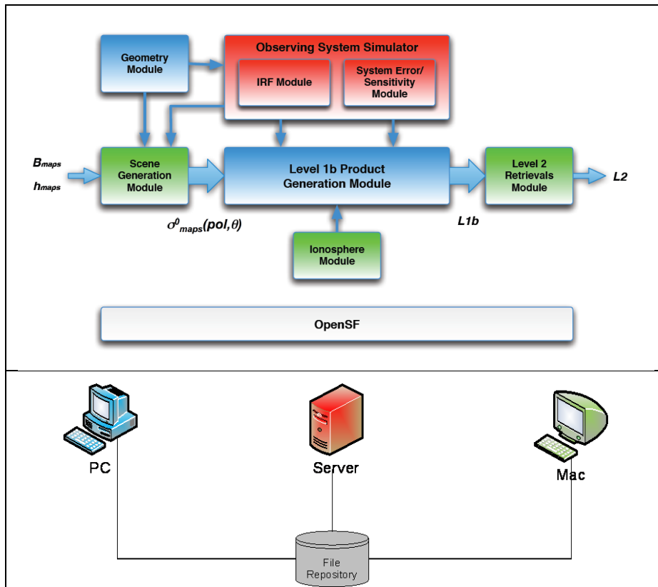
Figure 4-138: Outline of a simulation scenario
