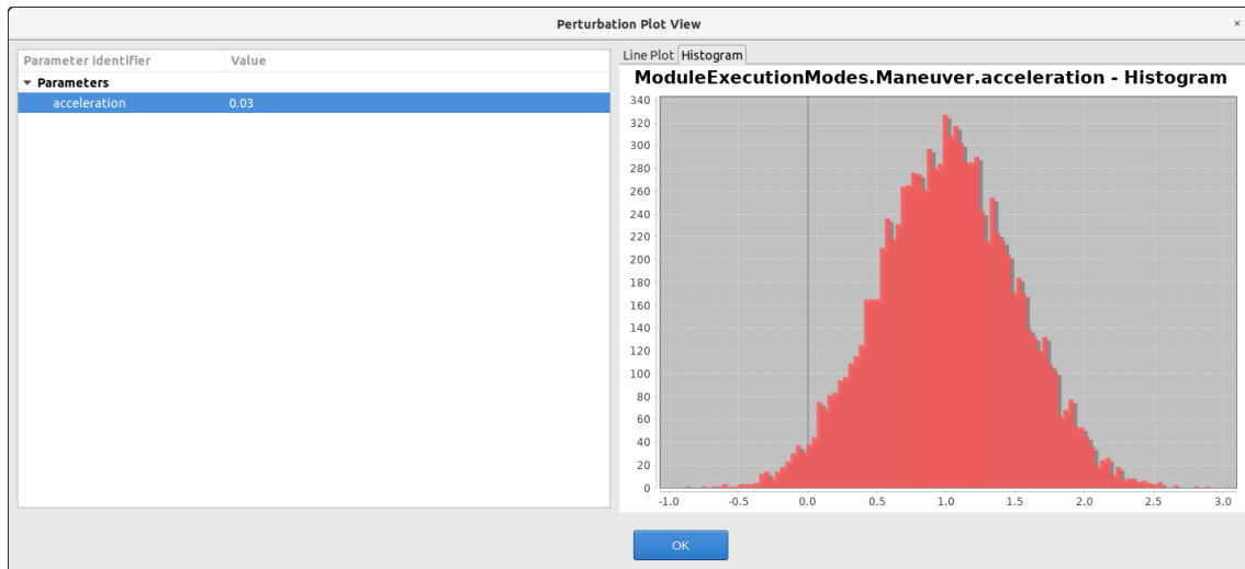
Figure 4-102: Histogram chart for a random parameter perturbation
