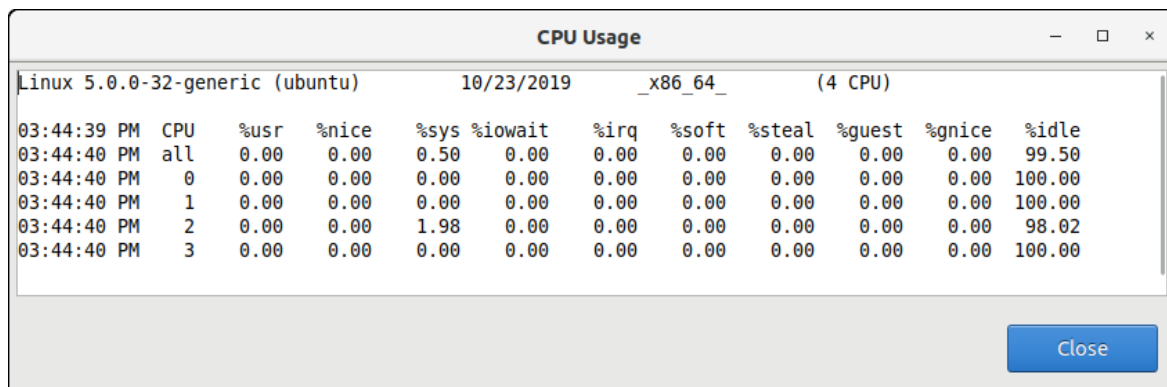
Figure 4-154: CPU Core Usage view
