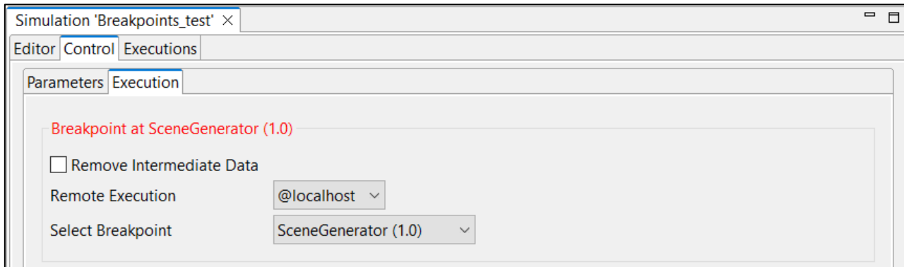
Figure 4-86: Breakpoint scheduling interface
