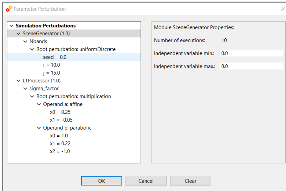
Figure 4-96: specific view of perturbations at module level
