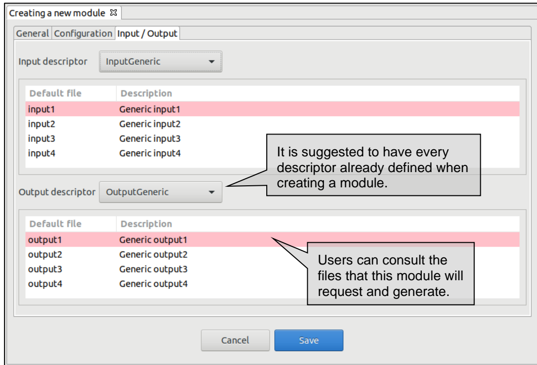
Figure 4-37: Module input/output specification
