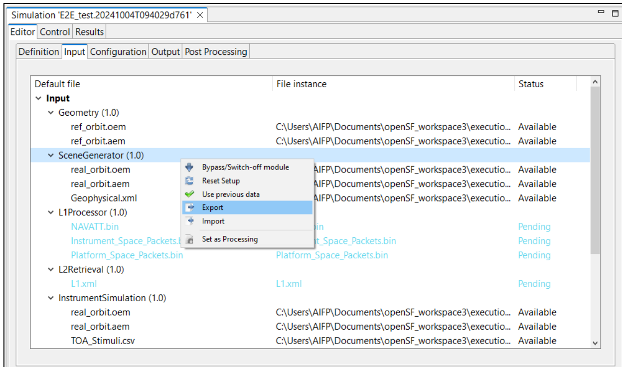
Figure 4-136: Export module from the Simulation Result view
