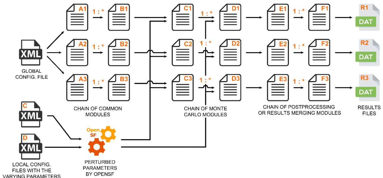
Figure 4-112: Monte Carlo chain in combined mode
