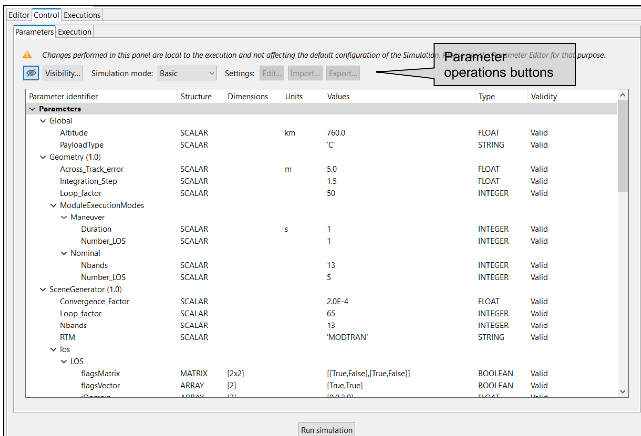
Figure 4-55: Simulation parameters definition
