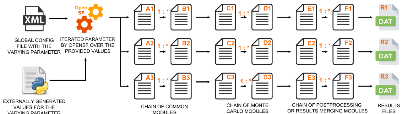
Figure 4-113: MC with a global parameter
