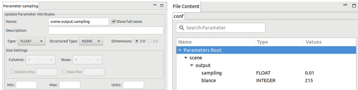
Figure 4-10: An example of a parameter and groups, in the parameter edition (left) and file (right) views
