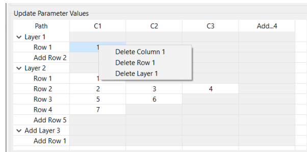
Figure 4-15: Context menu right-clicking on a cell in the values editor.
