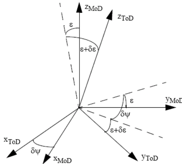
Figure 7: Transformation between MoD and ToD reference frames
