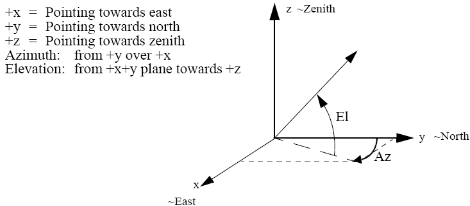
Figure 15: Topocentric direction
