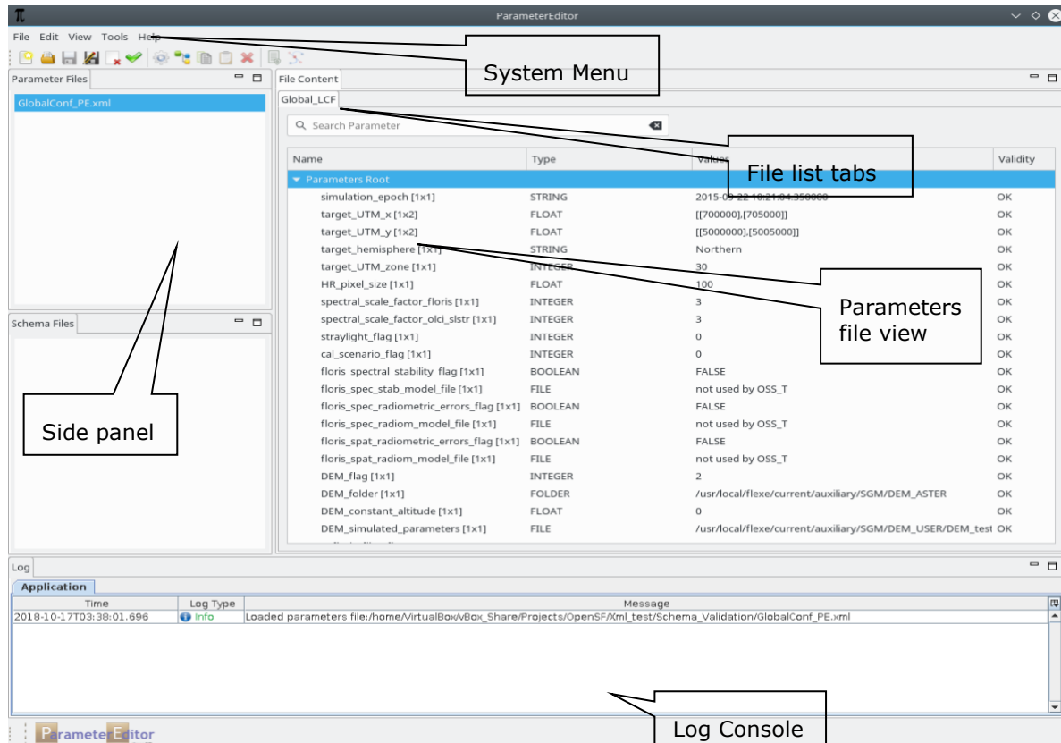
Figure 2: ParameterEditor Main Window Appearance
