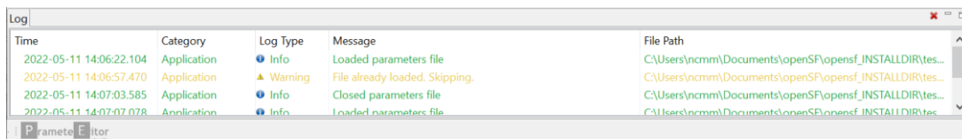
Figure 17: Log Console
