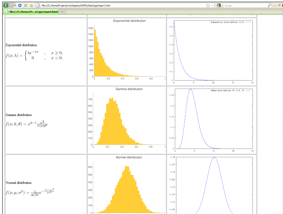
Figure 4-61: Web browser as openSF product tool
