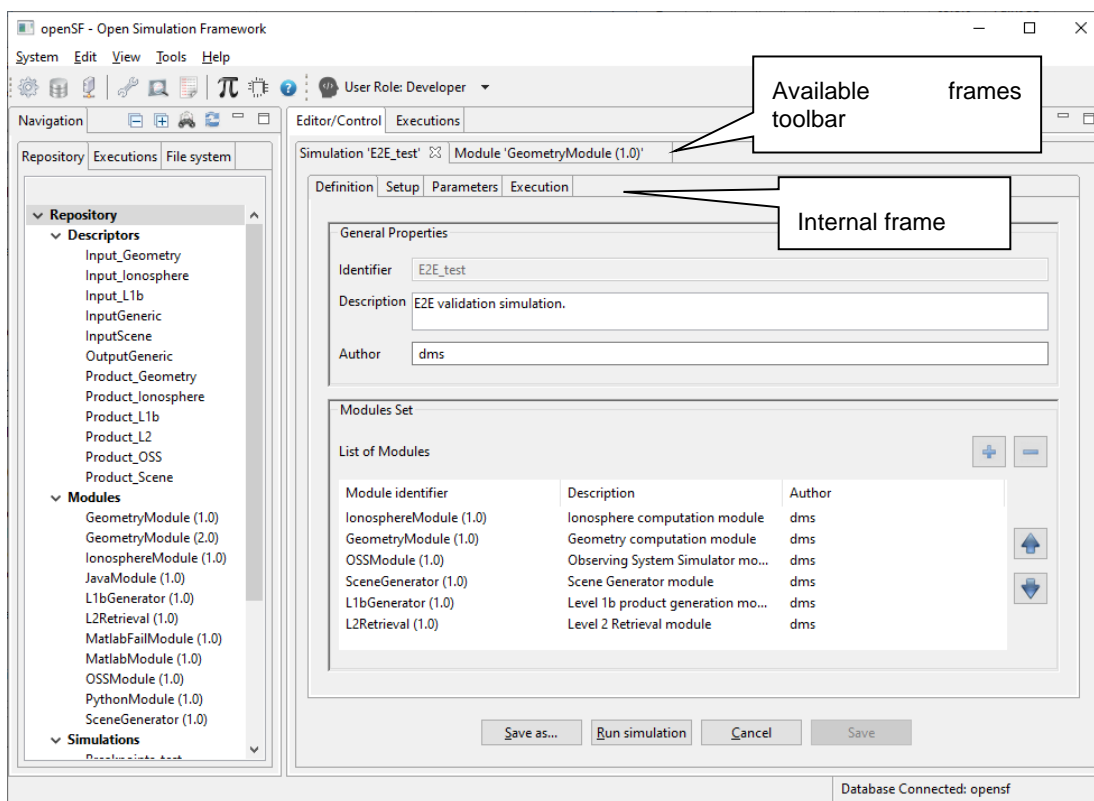
Figure 4-2: Main window appearance showing internal frames and scroll bars
