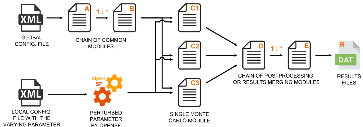
Figure 4-103: Monte Carlo chain in statistical mode
