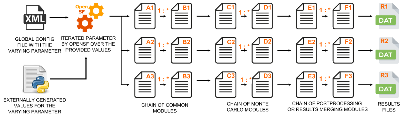
Figure 4-105: MC with a global parameter
