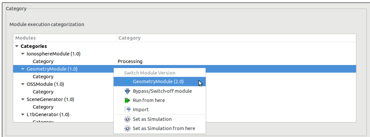
Figure 4-66: Switch module version
