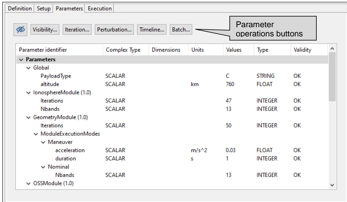
Figure 4-44: Simulation parameters definition
