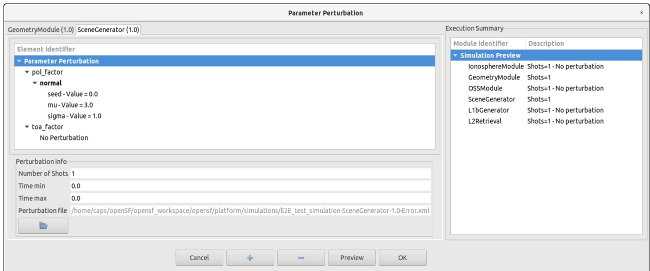
Figure 4-85: Complex perturbation function
