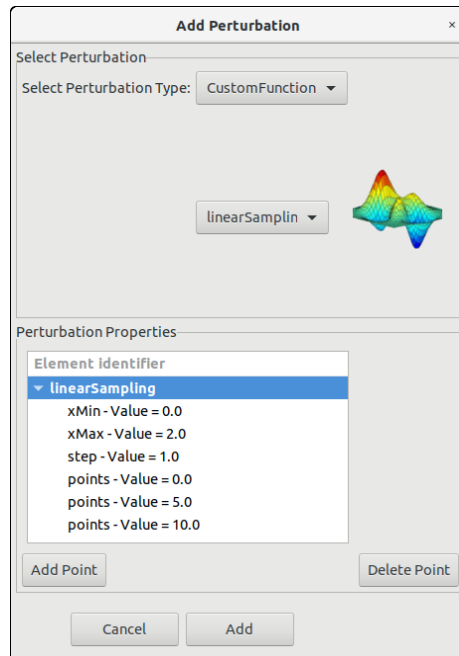
Figure 4-92: Function with variable number of properties (points)
