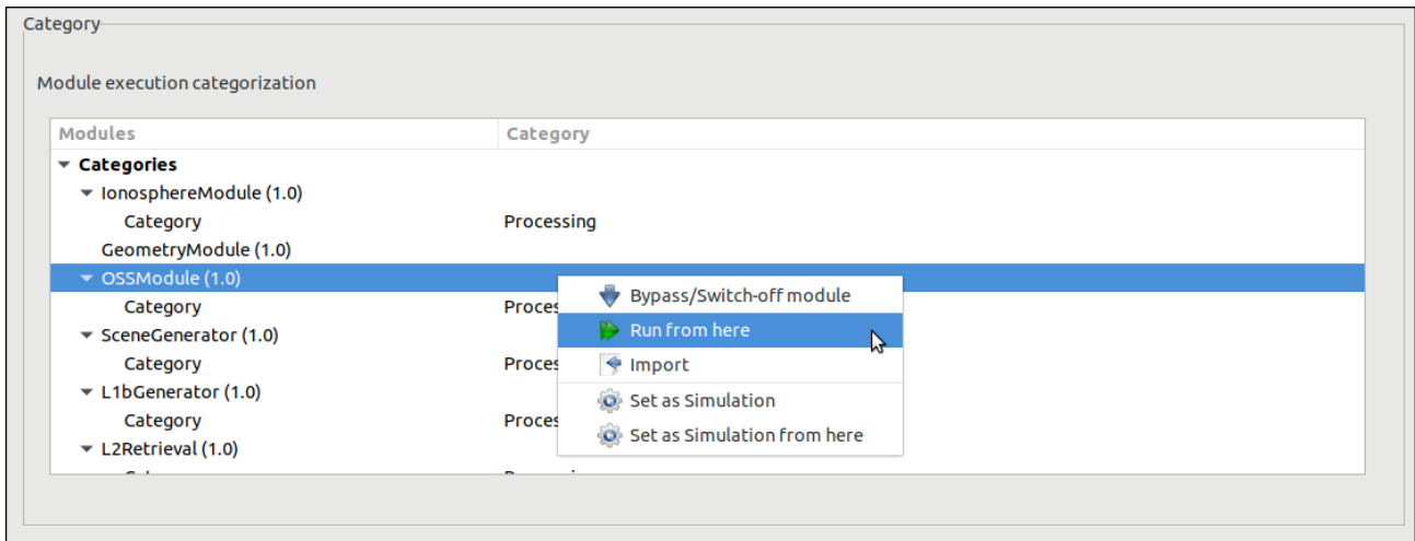
Figure 4-71: Run simulation from a given module
