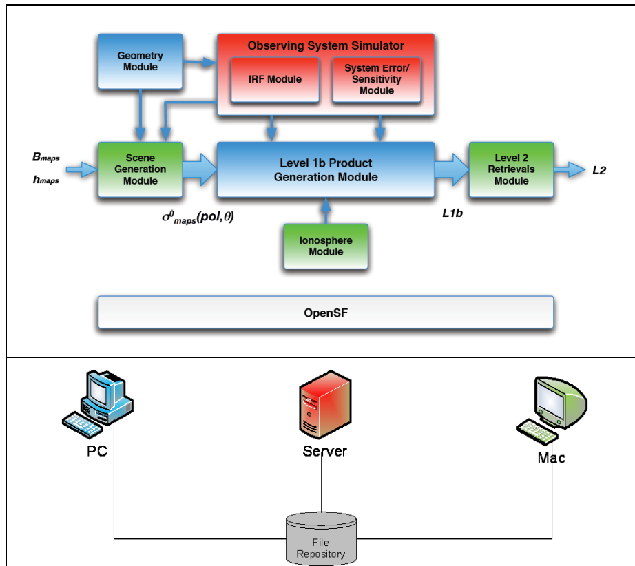
Figure 4-123: Outline of a simulation scenario
