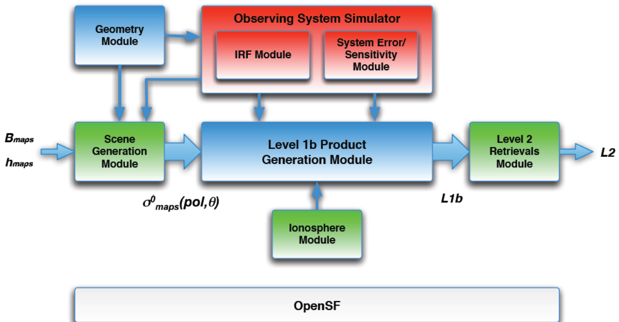
Figure 7-1: Outline of a test simulation scenario
