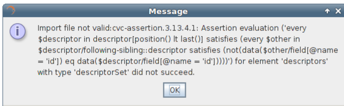
Figure 4-21: Database import XML definition error
