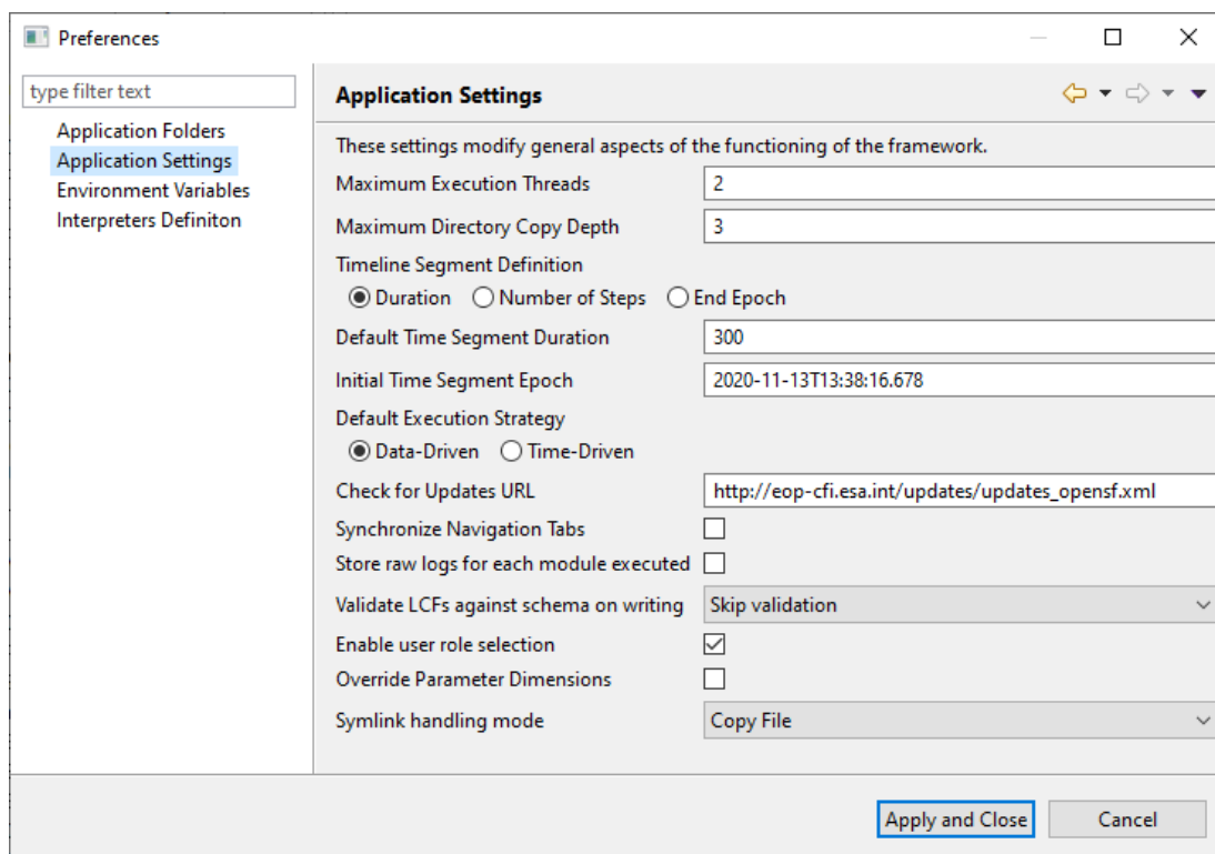
Figure 4-130: System Applications settings
