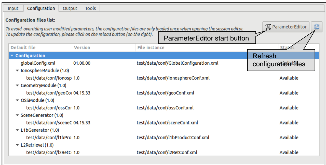
Figure 4-42: Configuration files definition
