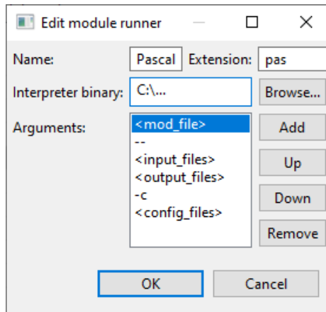
Figure 4-134 User-defined interpreter definition
