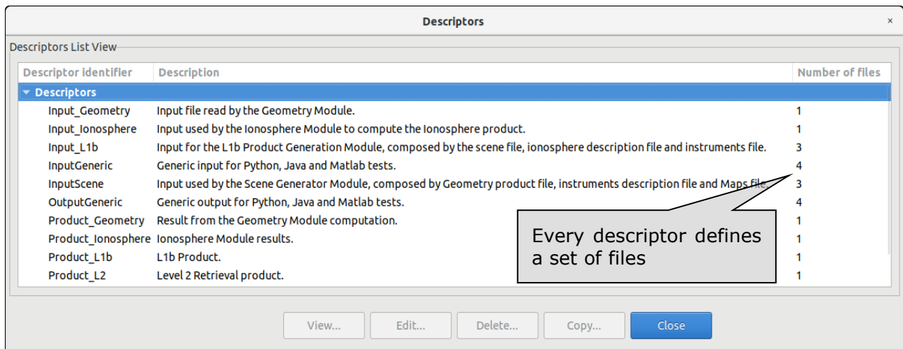
Figure 4-25: Descriptors list view
