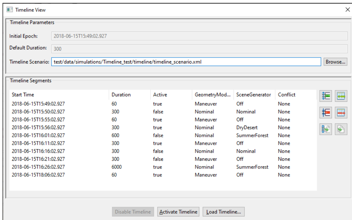
Figure 4-101: Timeline management view
